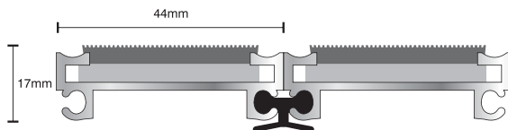
a-mats Hygiene-Plus 17mm with SBM 10 Black inserts
